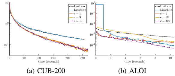
Figure 4. Optimality gap for CUB-200-2011 and ALOI
